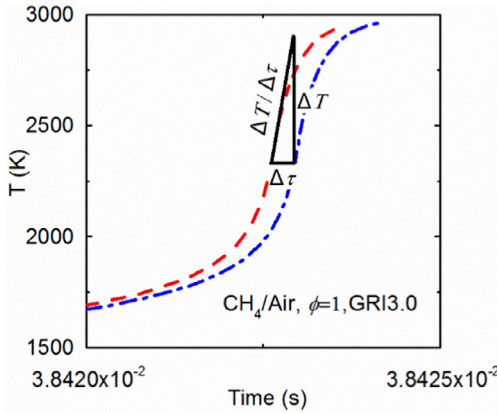
Fig. 6. Relations between changes of the ignition delay \tau and temperature at ignition due to perturbation of the rate constant.
