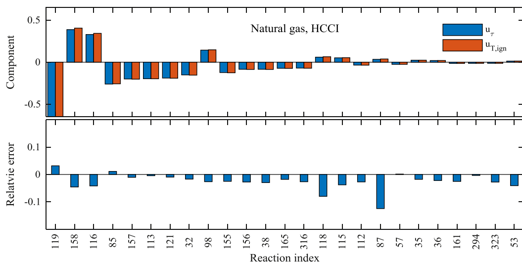
Fig. 7. Components of the sensitivity direction for IDT in the HCCI case and the component-wise relative differences between u_T and u_{T, \text{ign}} .
