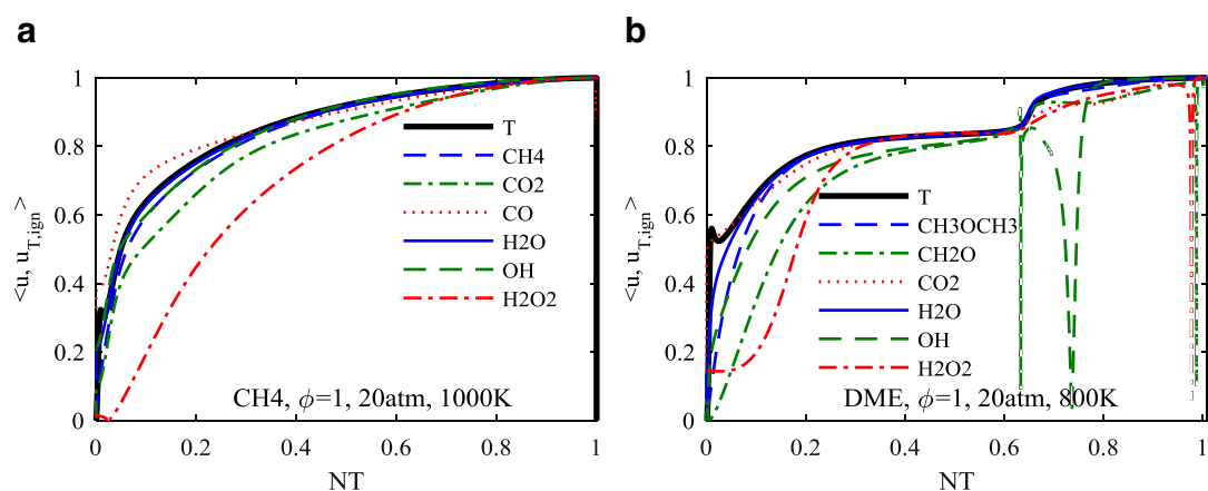
Fig. 2. Evolutions of the inner product (absolute value) between the sensitivity directions of composition and \mathbf{u}_{T, \text{ign}} .
