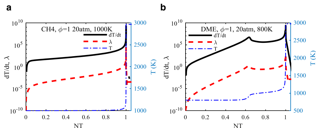
Fig. 1. Evolution of temperature, its rate of change, and the magnitude of its sensitivity vector to kinetic parameters against the normalized time. The unit of dT/dt is K/s . The IDT is 38.4 ms in (a) and 0.7 ms in (b).
