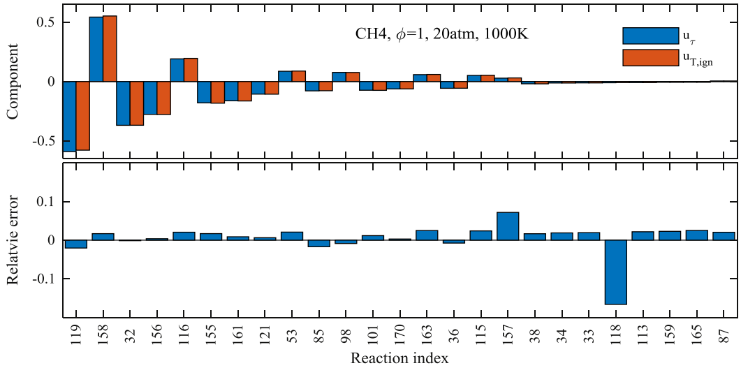
Fig. 5. Components of the sensitivity direction for IDT and the component-wise relative differences between u_\tau and u_{T, \text{ign}} .
