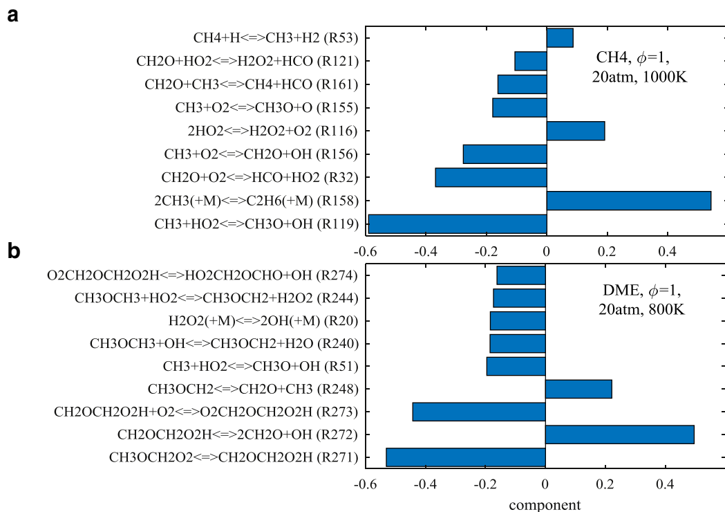
Fig. 3. The most sensitive reactions for temperature at the ignition point.
